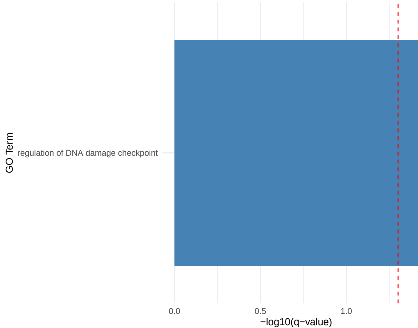
Pattern 1 Top Enriched GO Terms
