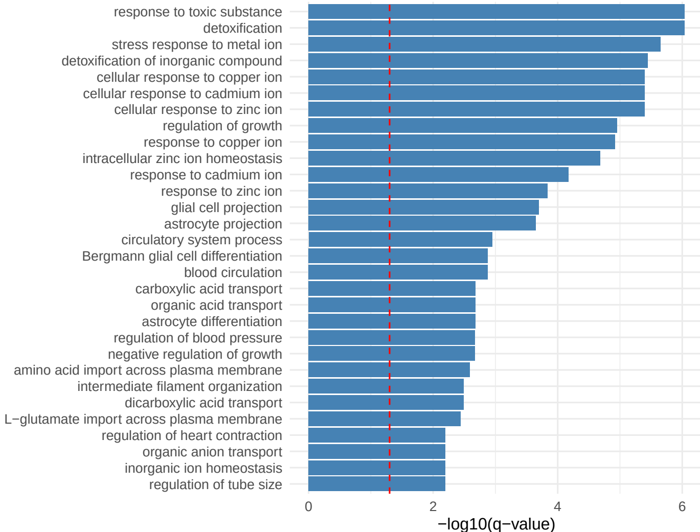
Pattern 20 Top Enriched GO Terms
