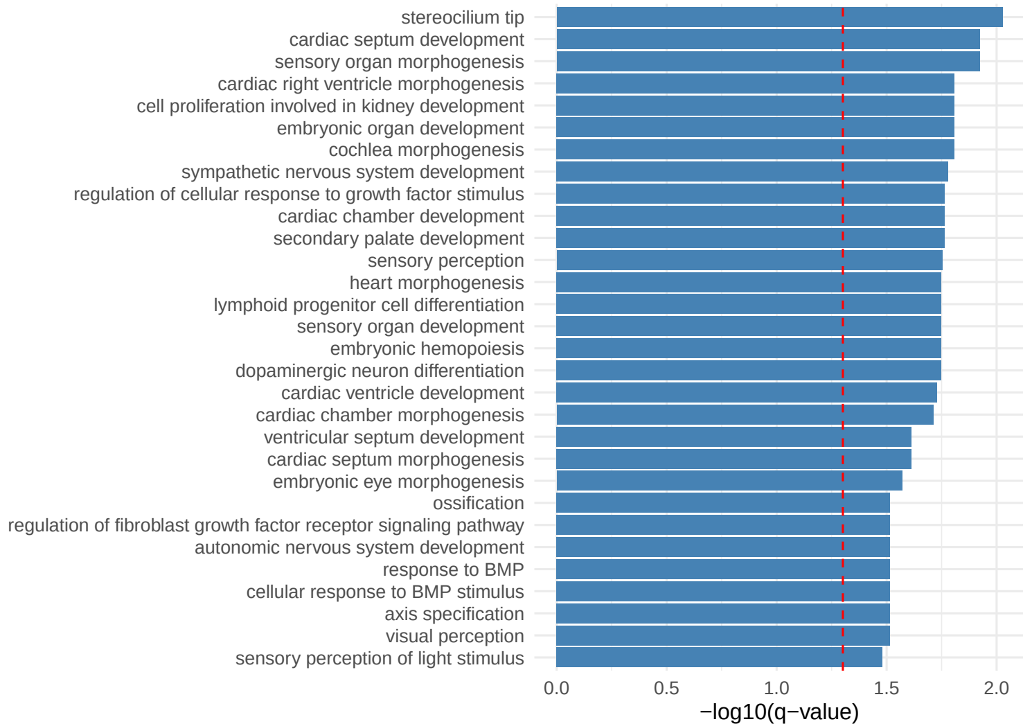
Pattern 24 Top Enriched GO Terms
