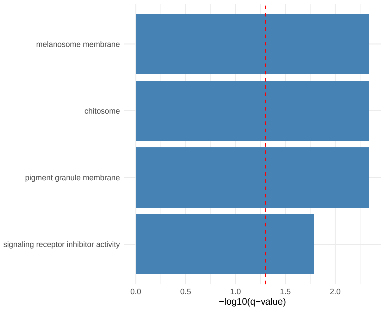
Pattern 30 Top Enriched GO Terms
