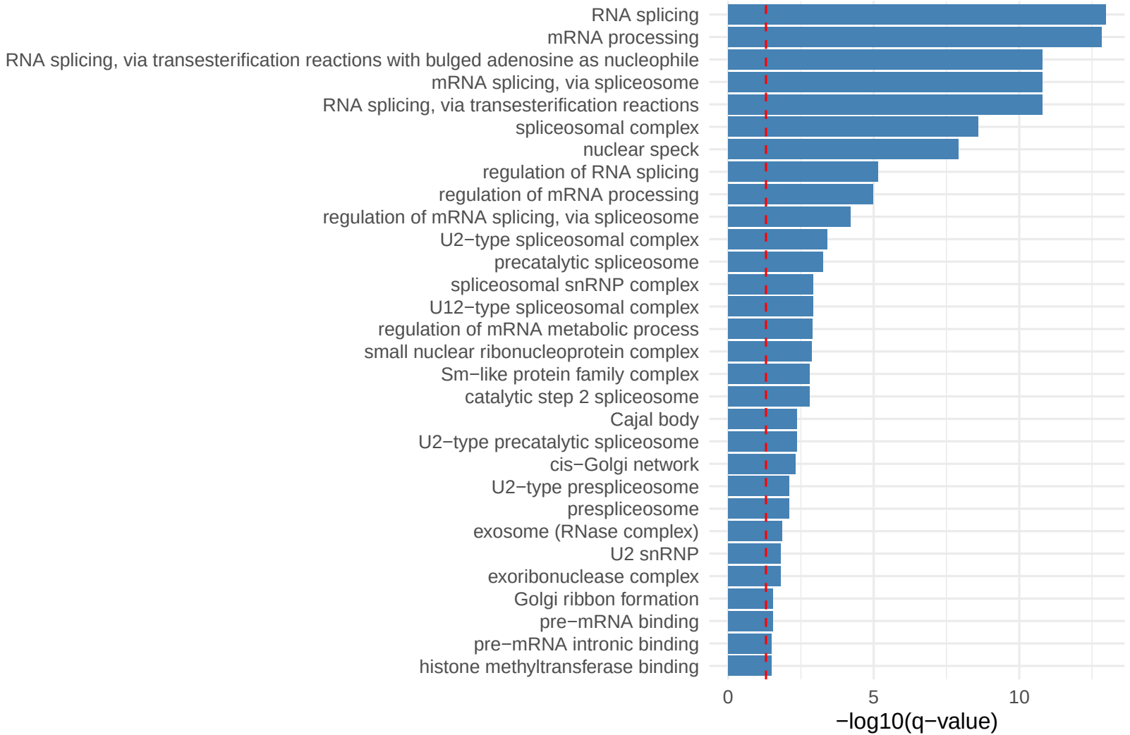
Pattern 33 Top Enriched GO Terms
