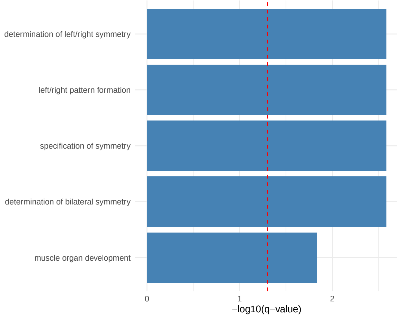
Pattern 42 Top Enriched GO Terms
