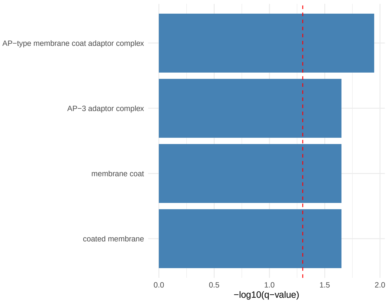
Pattern 43 Top Enriched GO Terms
