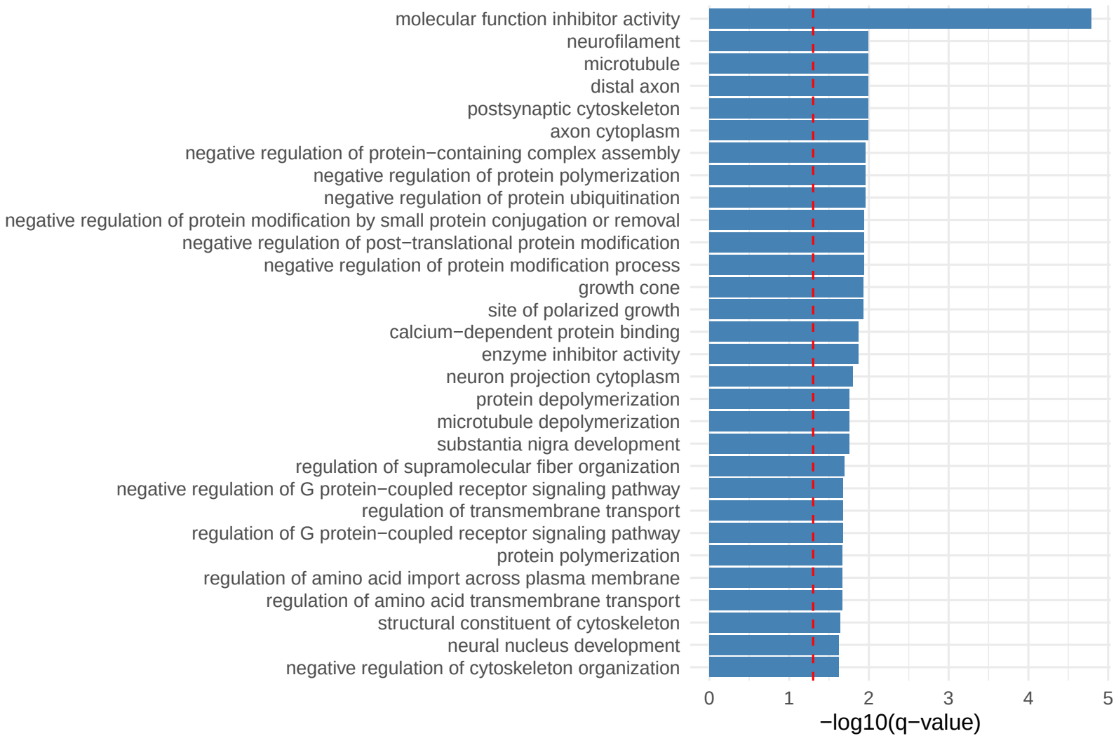
Pattern 45 Top Enriched GO Terms
