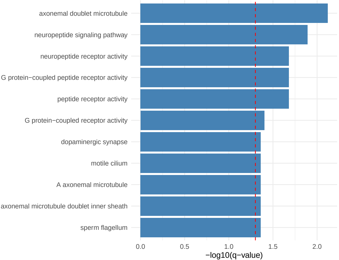
Pattern 47 Top Enriched GO Terms
