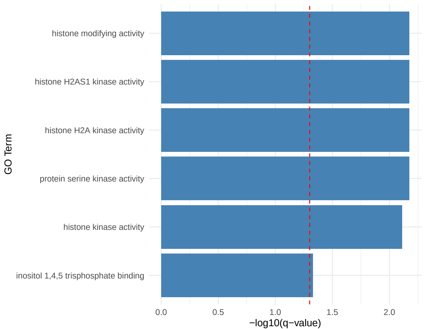
Pattern 51 Top Enriched GO Terms
