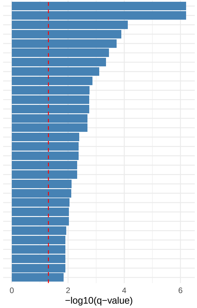
Pattern 60 Top Enriched GO Terms
