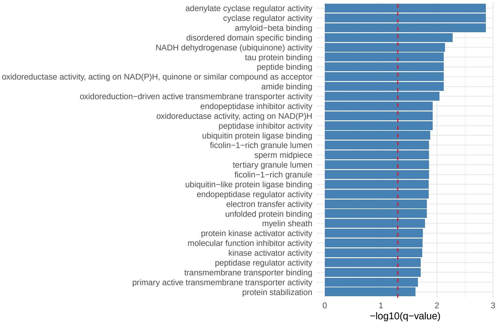
Pattern 62 Top Enriched GO Terms
