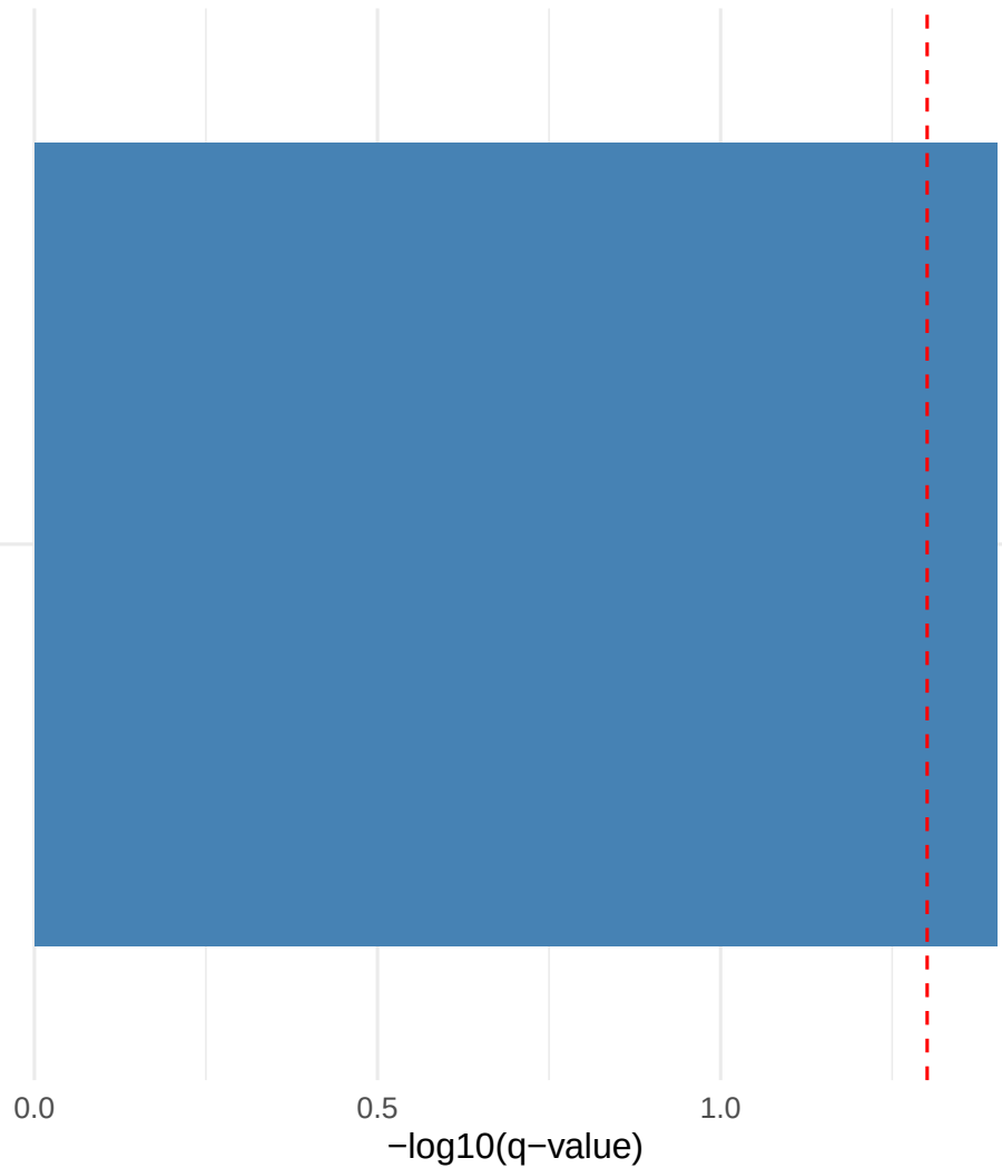
Pattern 66 Top Enriched GO Terms
