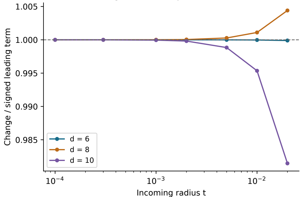
Convergence of the proved coefficient
