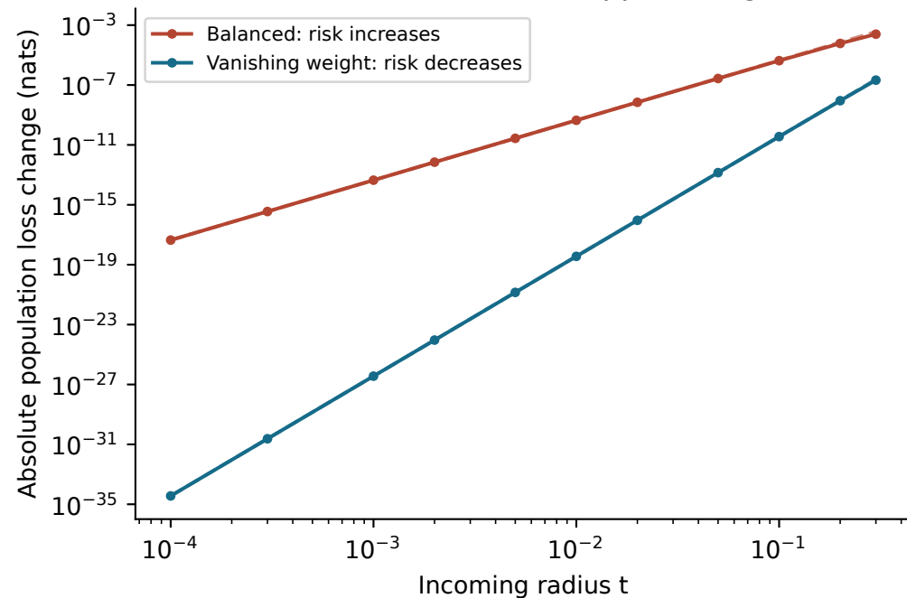
Same two-child width; opposite signs
