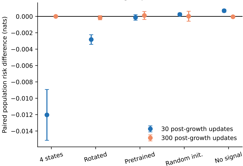
Direction advantage: spectral minus random
