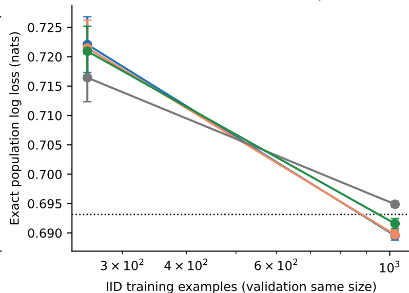
Rotated 8-dimensional inputs
