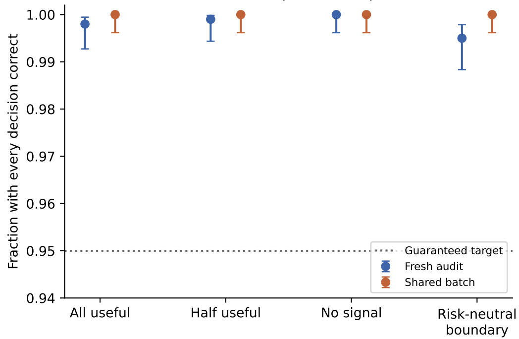
K = 16 ; 1,000 independent replications
