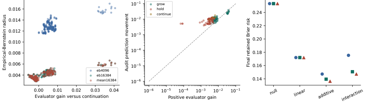
Figure 5: Measured evidence diagnostics. Left: the finite-bound radius versus evaluator gain over continuation for nonlinear residual proposals; the mean-gate radius is diagnostic only. Middle: audit prediction movement versus positive evaluator gain at the larger finite-bound audit; the dashed line is the Bayes-refit identity, not a fitted neural law. Right: final risk under small-audit finite bounds (blue), large-audit finite bounds (green), and the large-audit empirical-mean heuristic (red). All input-population quantities are Monte Carlo estimates; decisions use sampled audit labels.
