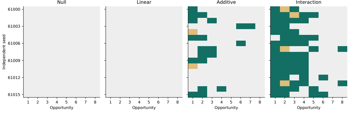
Figure 2: Every primary residual trajectory at the larger audit budget. Green means accepted growth; amber means accepted continuation; light gray means the incumbent parameters are held. Rows are the 16 prespecified seeds, columns the eight decision opportunities. An external opportunity schedule exists, but actions and accepted final capacity are data-dependent.
