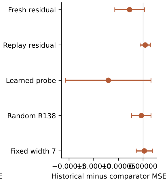
lowrank noiseless
