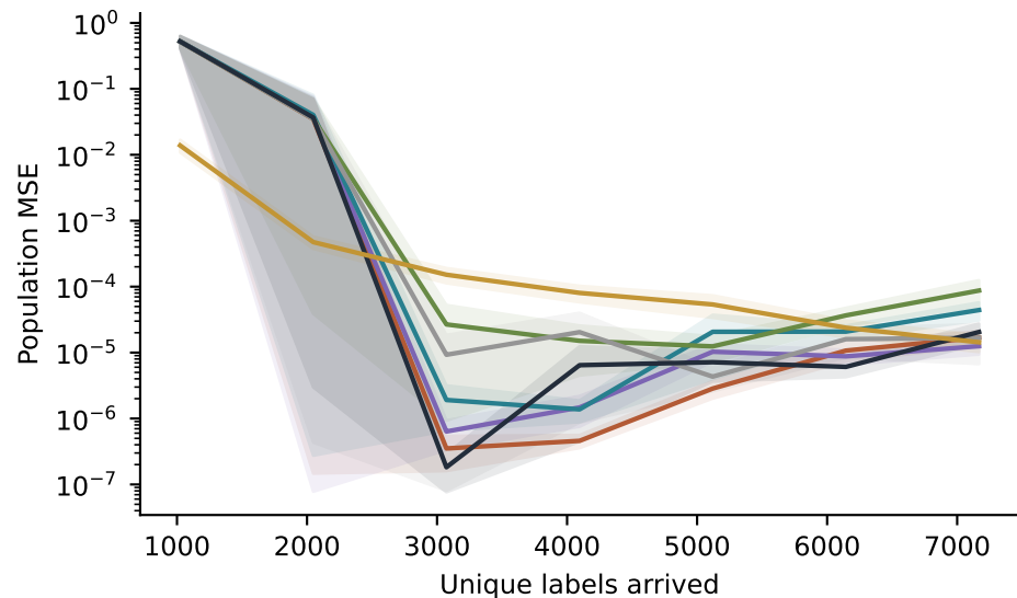
nonlinear
