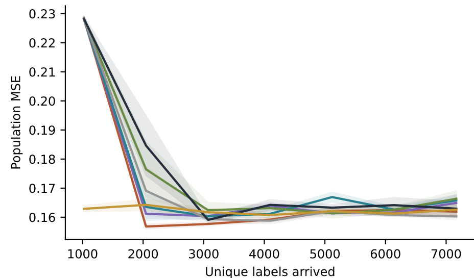
nonlinear
