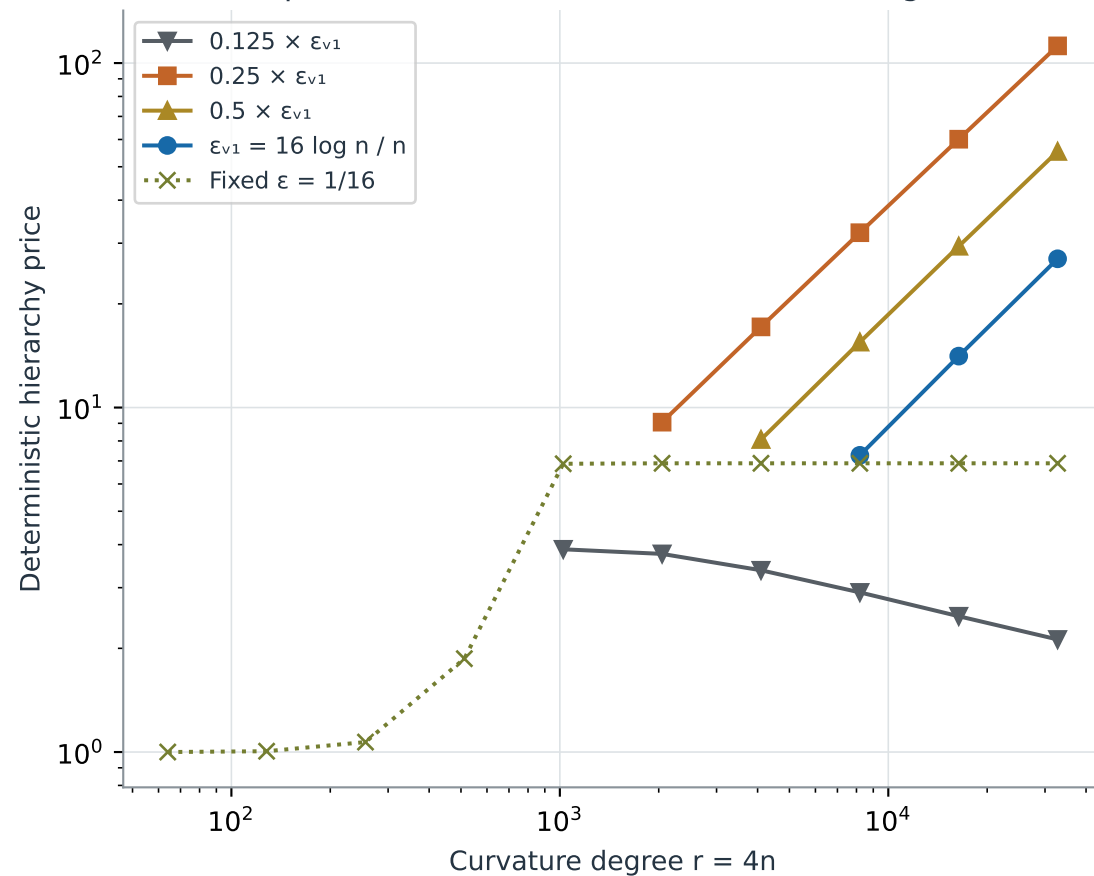
Equal masses: width matters at finite degree
