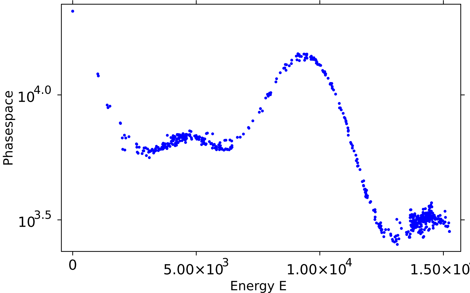
my 1-phonon phasespace
