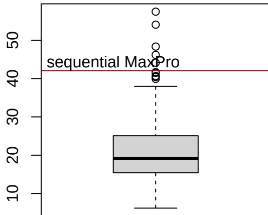
RMSE
