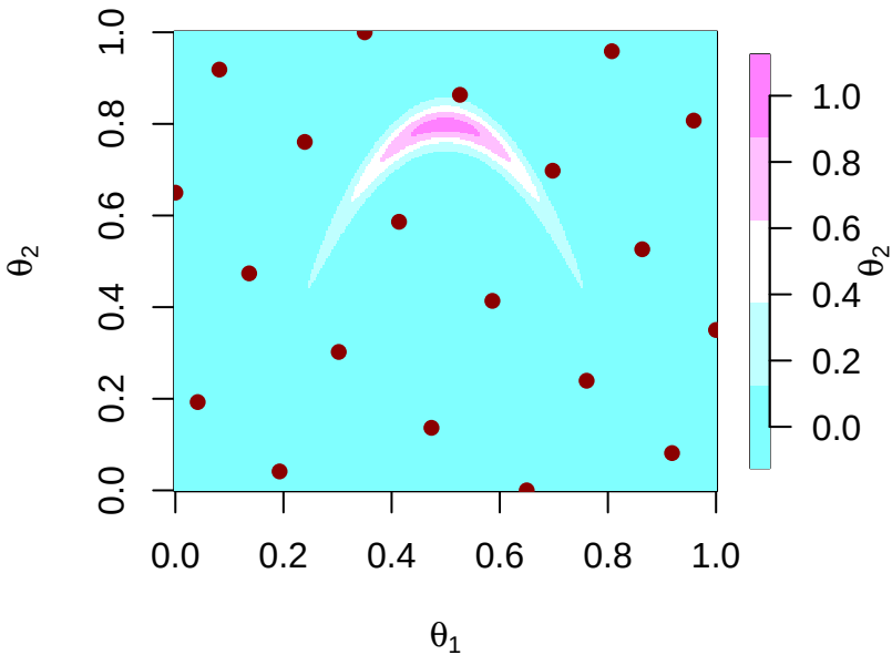
initial MaxPro design
