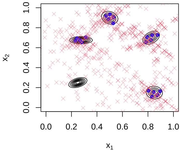
Population Quasi-Monte Carlo
