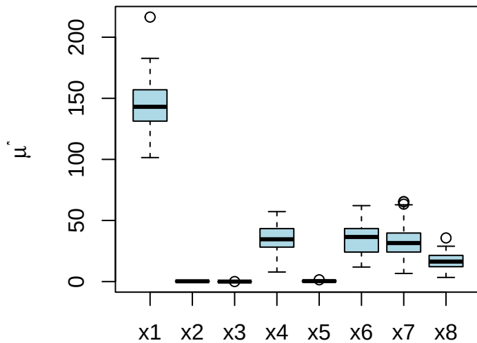
Morris Screening Design
