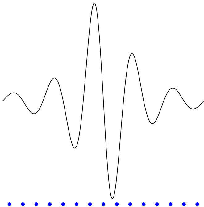
Approximate a Rough Function
