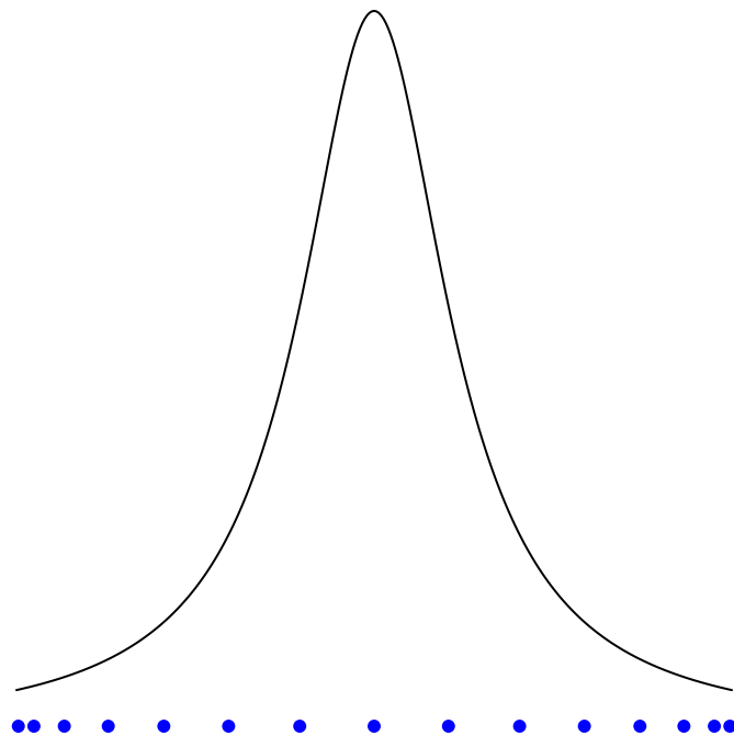
Approximate a Smooth Function
