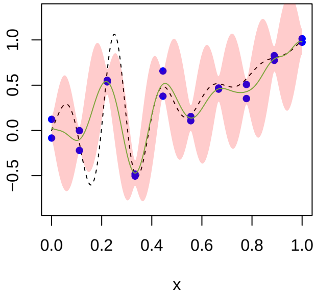
GP Regression (Equi-spaced)
