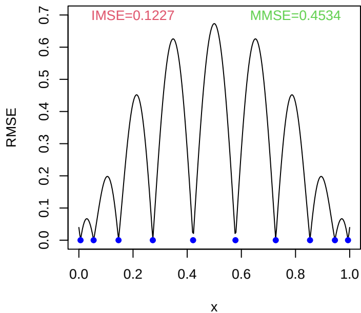
Chebyshev Design
