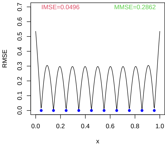
IMSE-optimal Design
