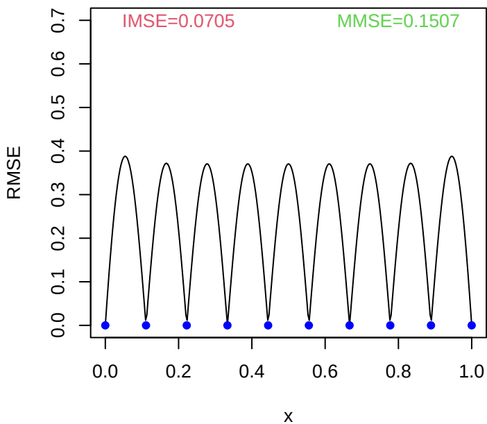
Equi-spaced Design
