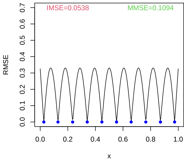
MMSE-optimal Design
