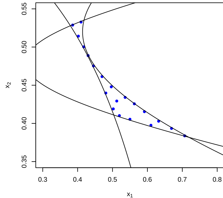
MaxPro design
