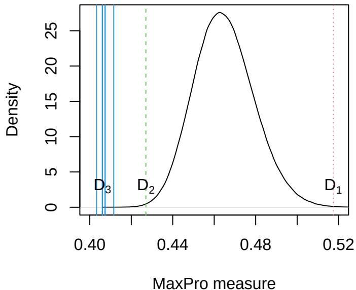
MaxPro criterion for 18-run designs
