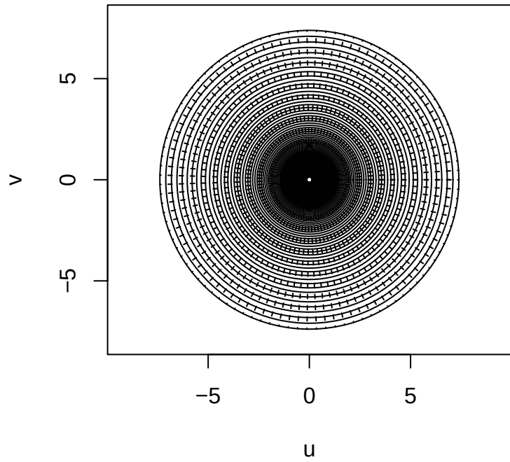
Image After w=e^z
