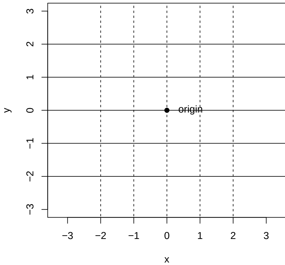
Complex Plane
