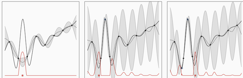
Figure 5: Two iterations of the expected improvement minimization algorithm on a test function
