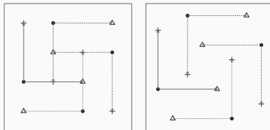
Figure 3: Maximum one-factor-at-a-time design (left) and maximum one-factor-at-a-time design with projection (right)
