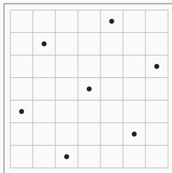
Figure 1: Maximin Latin hypercube sampling design
