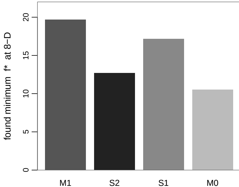
8-D: all fail (curse of dimensionality)
