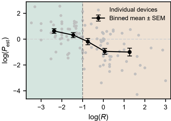
Internal resistance vs performance
