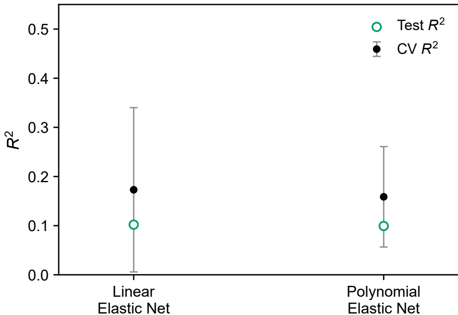
Linear vs polynomial descriptor model
