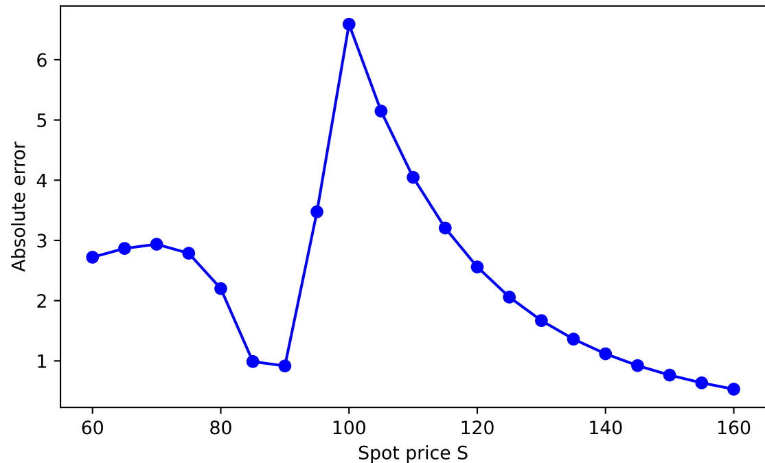
Heston absolute error (MAE=2.3573)
