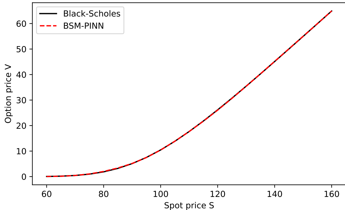
BSM-PINN vs Analytical
