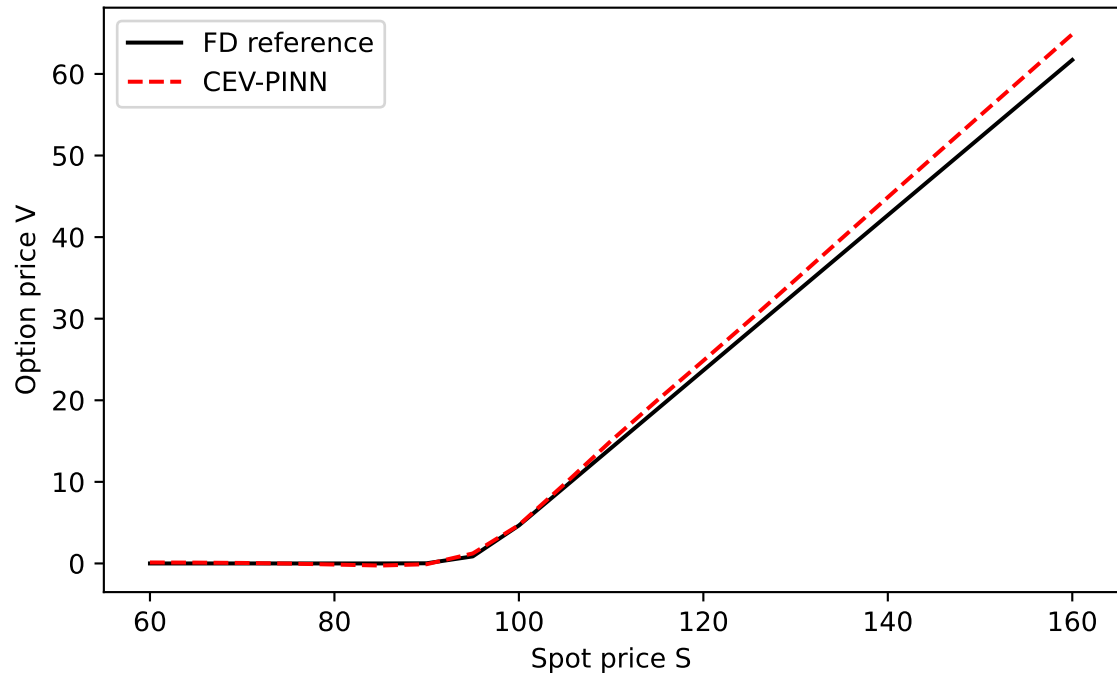
CEV-PINN vs FD (beta=0.5)
