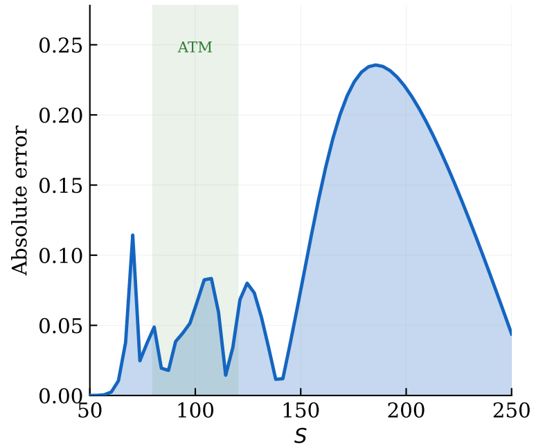
Heston
