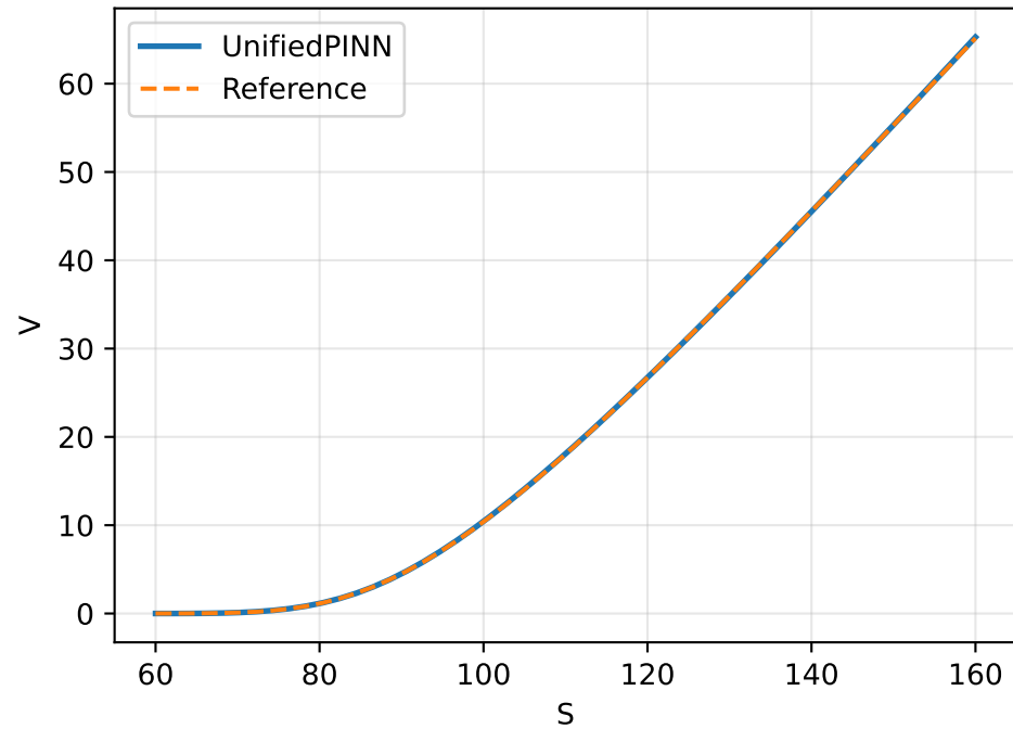
Heston
