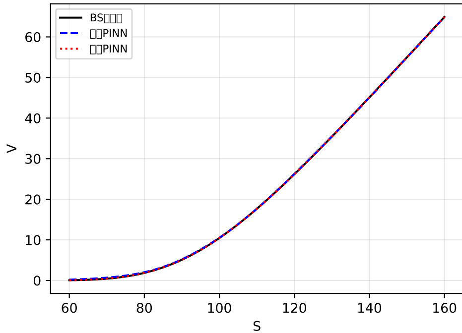
BSM ( \sigma=0.20 )
