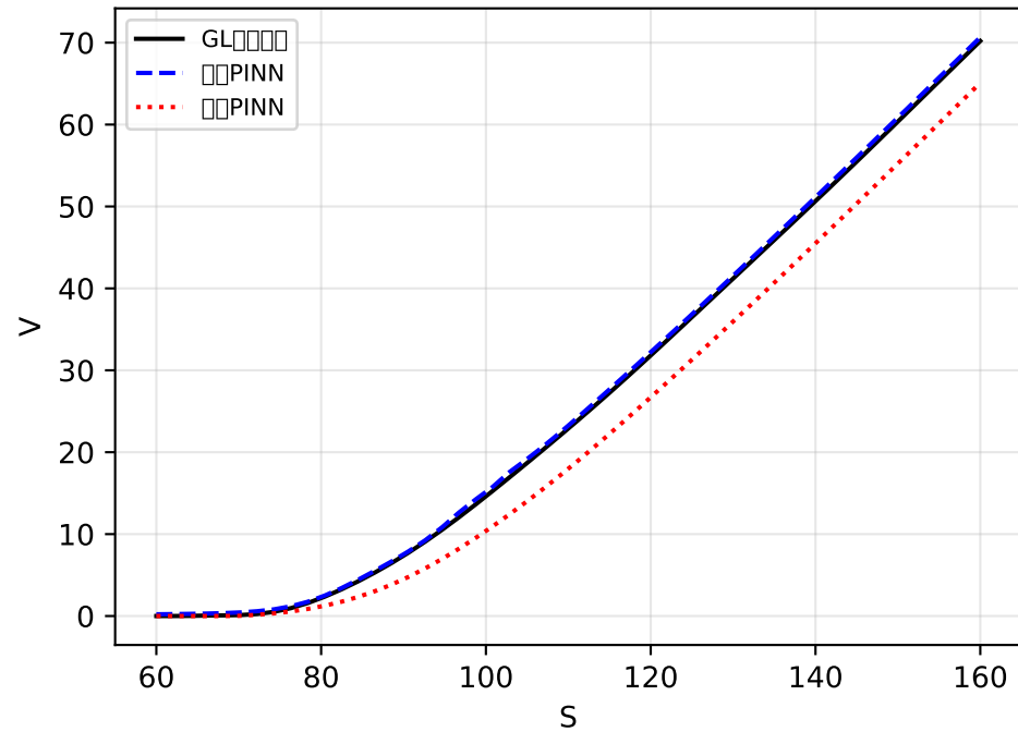
Heston ( \kappa=2, \xi=0.3, \rho=-0.7 )
