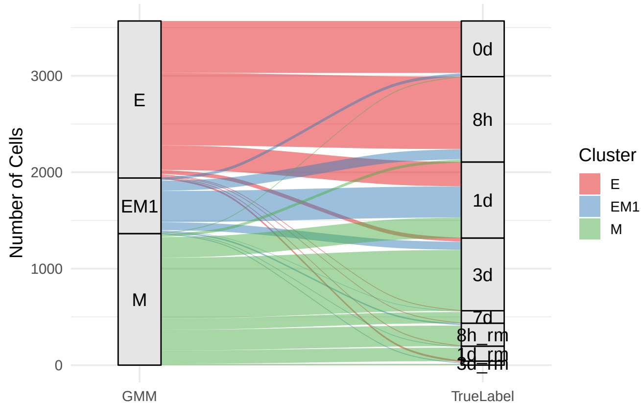
Sankey Diagram: GMM Cluster vs True Cell Labels – A549_
