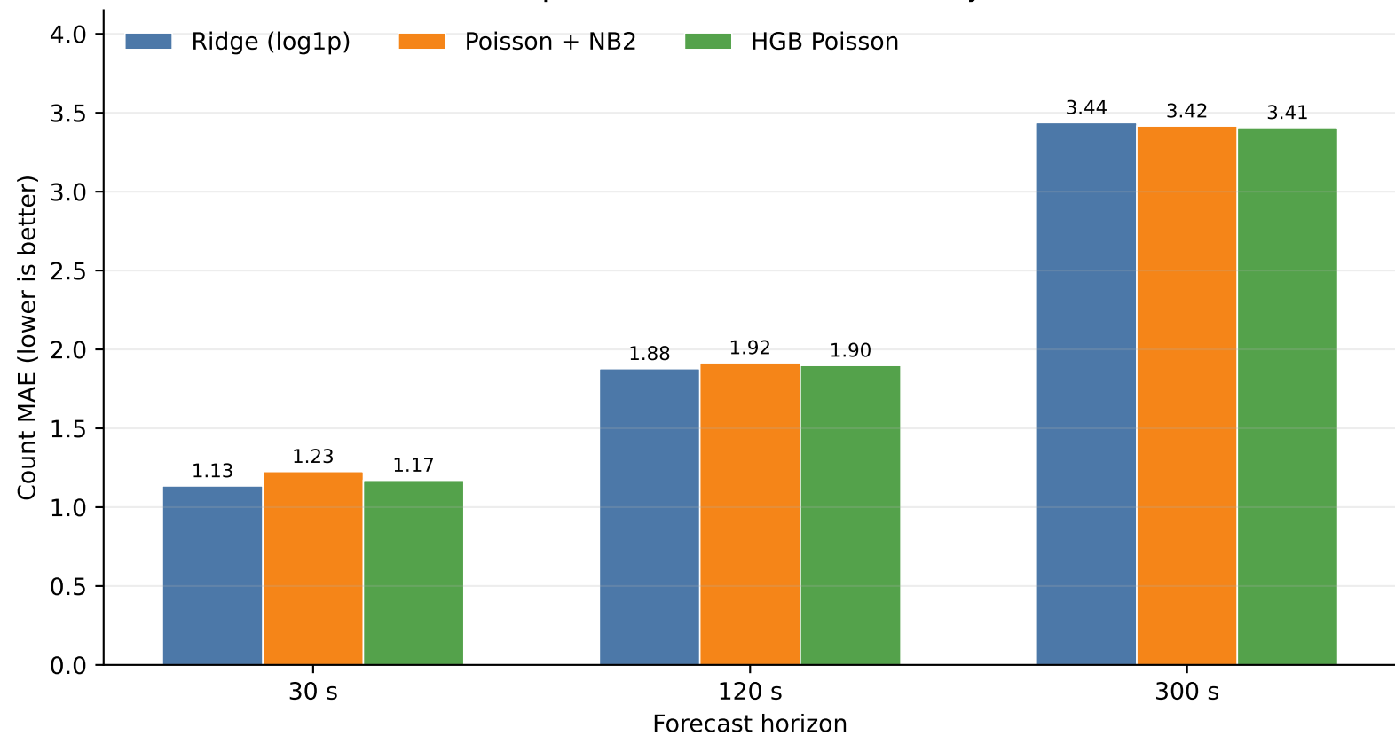
Point forecast performance on the final 8-day external set
