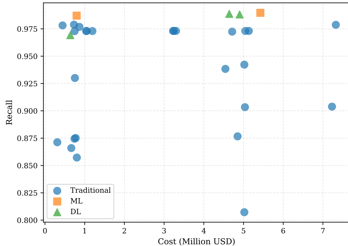
(b) Cost-Recall by Algorithm
