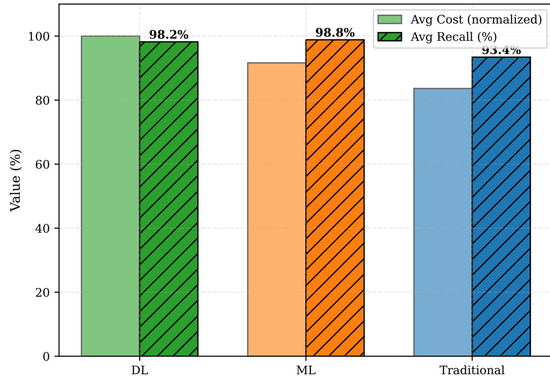
(b) Algorithm Performance Comparison
