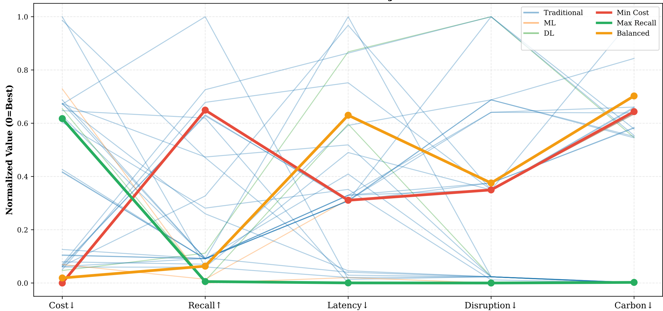
Parallel Coordinates: Multi-Objective Trade-offs
