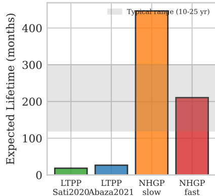
(c) Expected Pavement Lifetime
