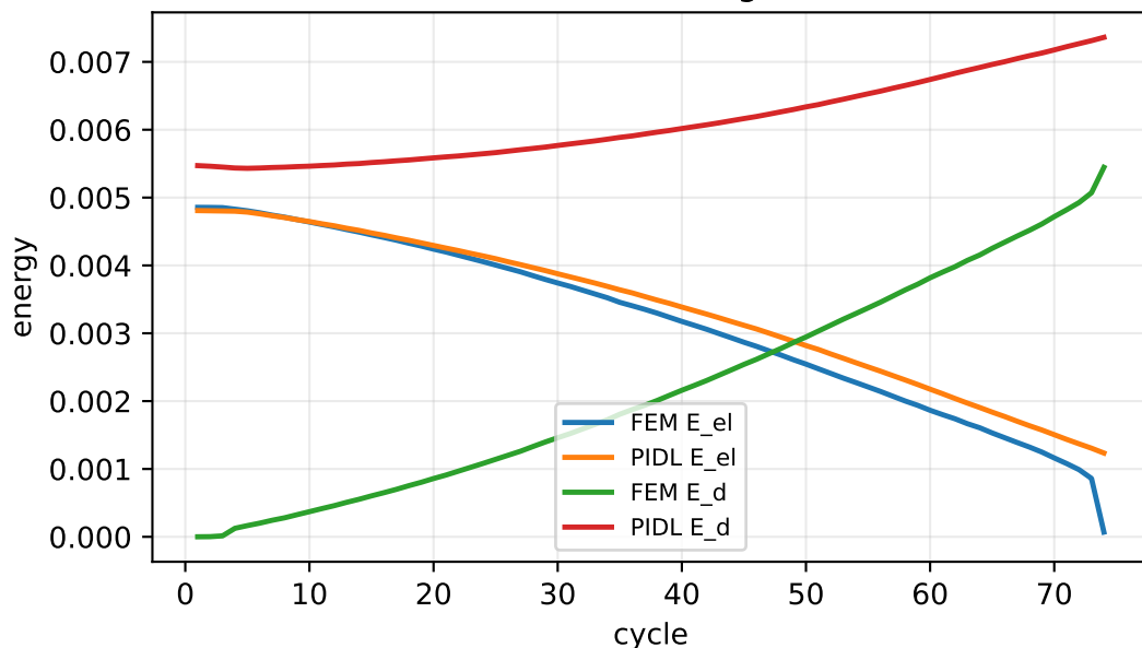
Fatigue-History Level
