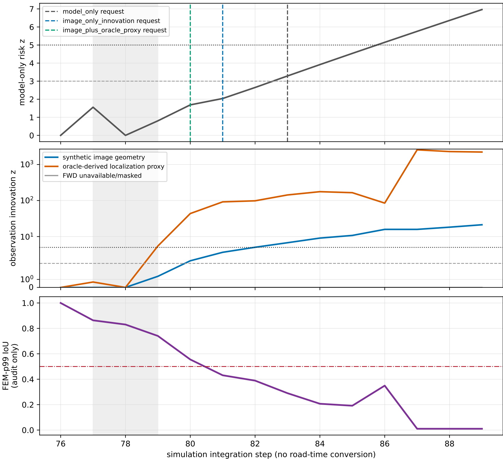
Model-only versus observation-innovation trigger single eta0 synthetic/oracle-derived diagnostic; FEM mechanism is audit-only
