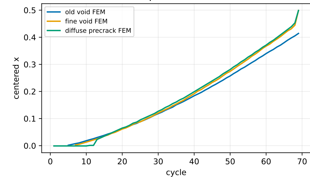
Crack-Tip Position d \geq 0.95
