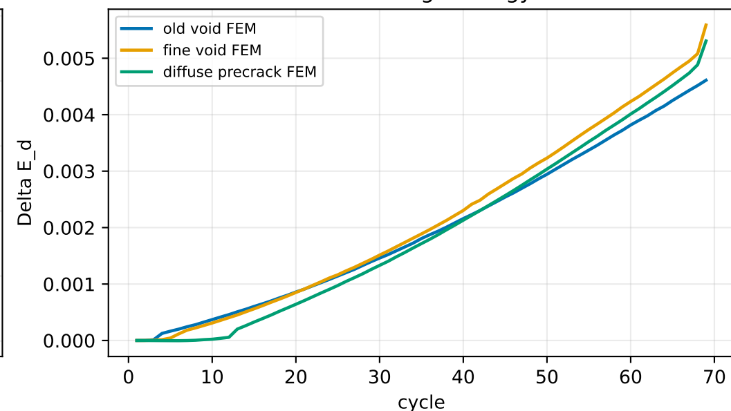
Minimum Fatigue Degradation
